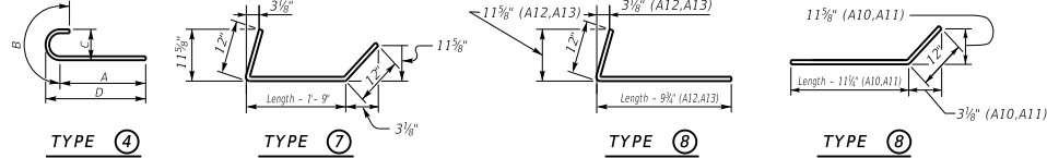
Reinforcement Details
